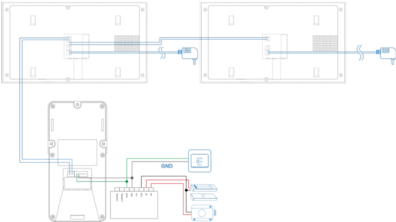
Image 1-7 Access Control Power Connection Diagram 1 Set Outdoor Station to 2 Set Indoor Monitor
